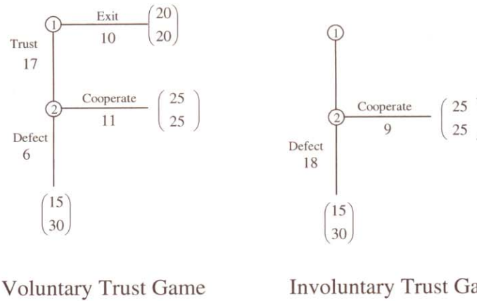
Figure 2. Frequency of Actions Chosen in McCabe, Rigdon, and Smith (2003)
