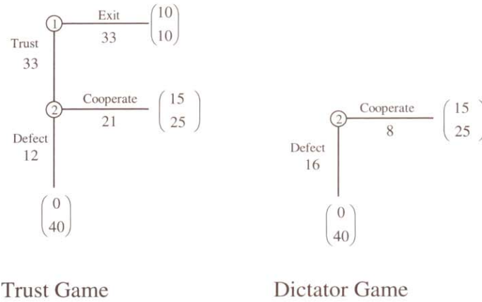
Figure 1. Frequency of Actions Chosen in Cox and Deck (2005, 2006)
