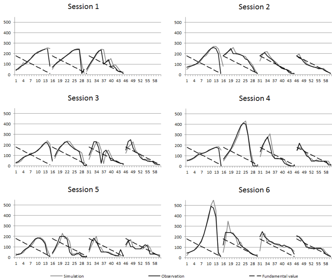
Figure A2. Observed and simulated average market price per session. Periods 1-15, 16-30, 31-45, and 46-60 correspond to markets 1, 2, 3, and 4, respectively.
