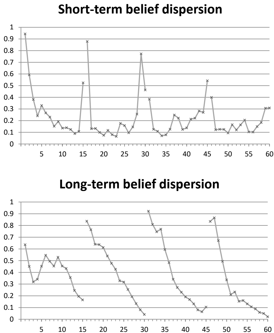
Figure A1. Average short-term and long-term belief dispersion, averaged over all sessions, each market separately.
