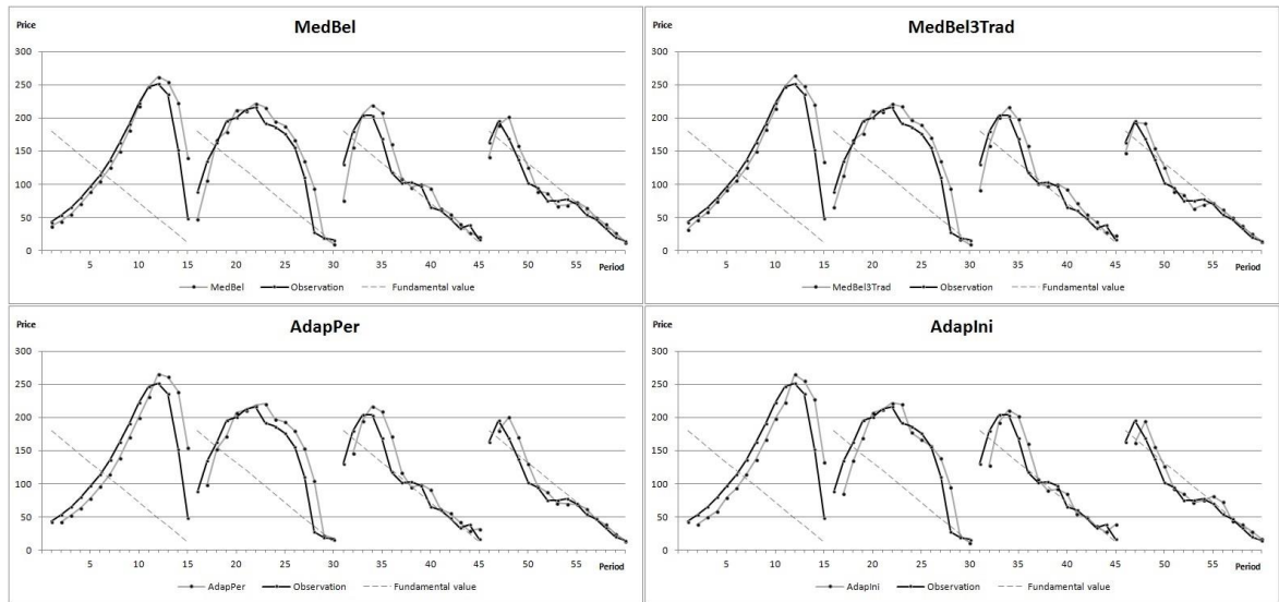
Figure A3. Observed and simulated average prices for the partial belief models MedBel , MedBel3Trad , AdapPer , and AdapIni
